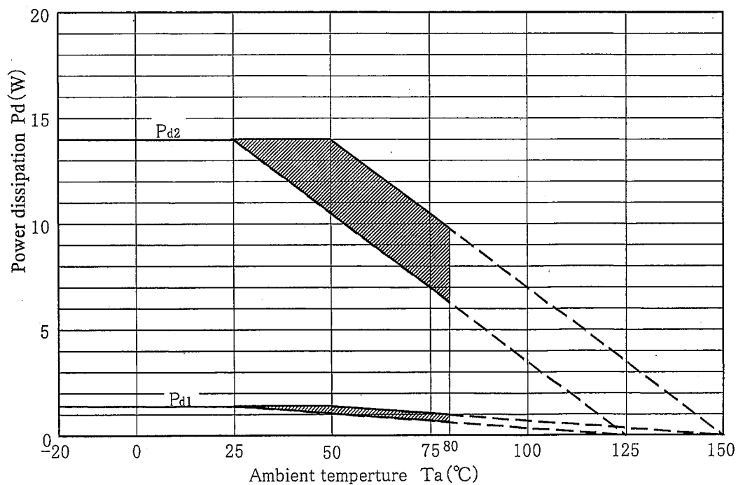
Fig. 1 Inner derating curve
