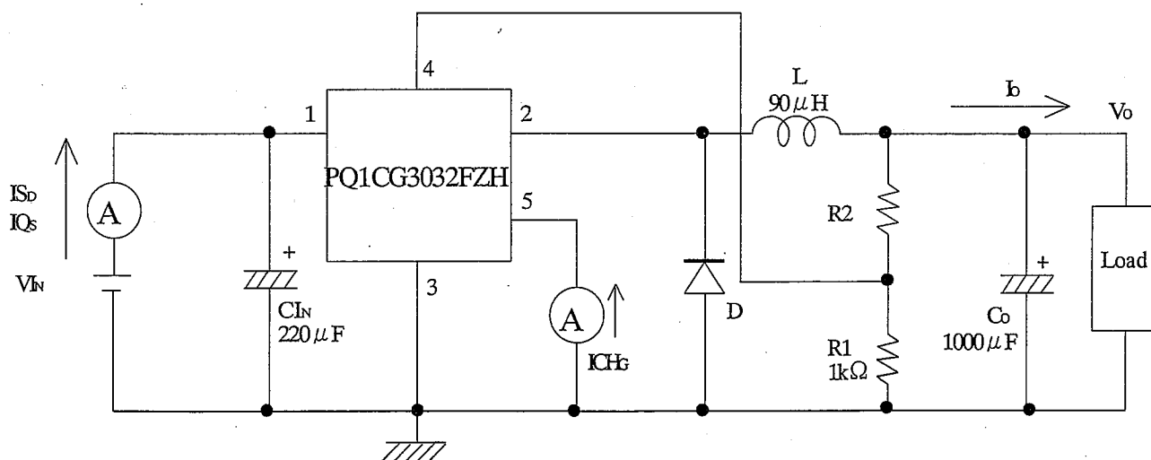
Fig. 2 Standard measuring circuit
