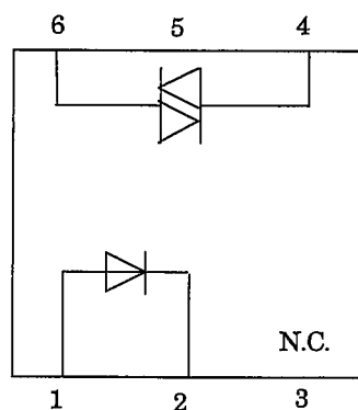
Pin Nos. and internal connection diagram
