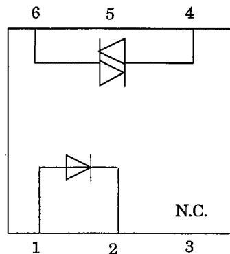
Pin Nos. and internal connection diagram
