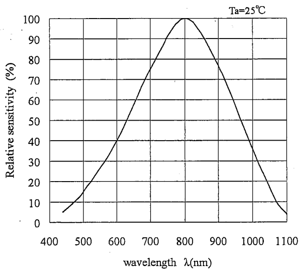
(3.4) Spectral sensitivity (reference)
