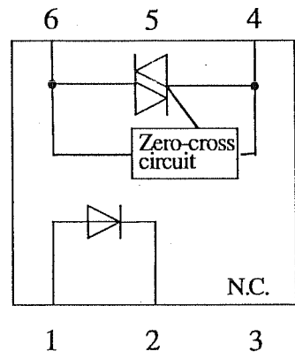
Pin Nos. and internal connection diagram
