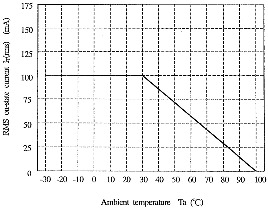
Fig.2 RMS on-state current I_f(\text{rms}) vs. ambient temperature
